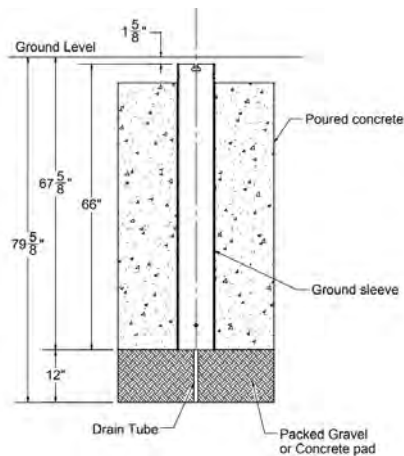
GROUND SLEEVE
